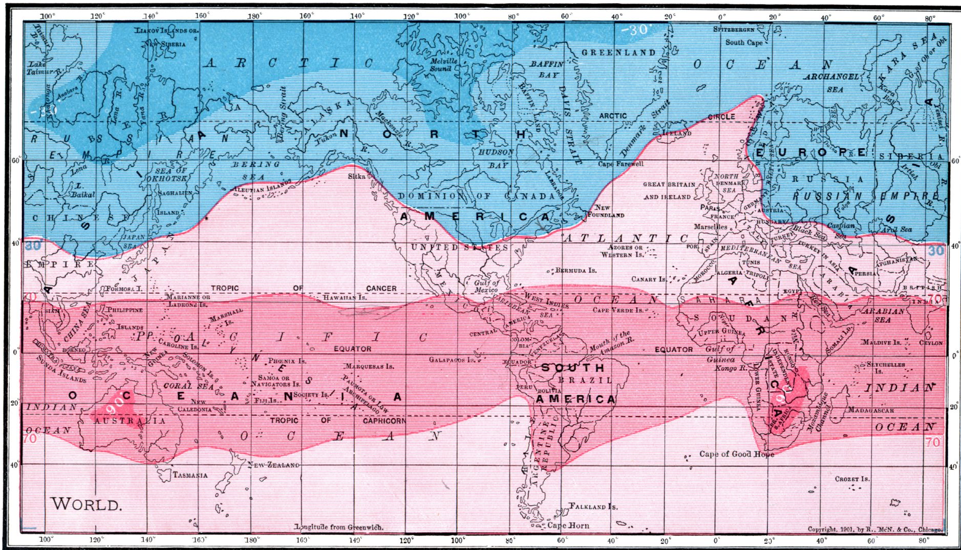
MAP SHOWING ISOTHERMS FOR JANUARY. (Fig. 77.)
