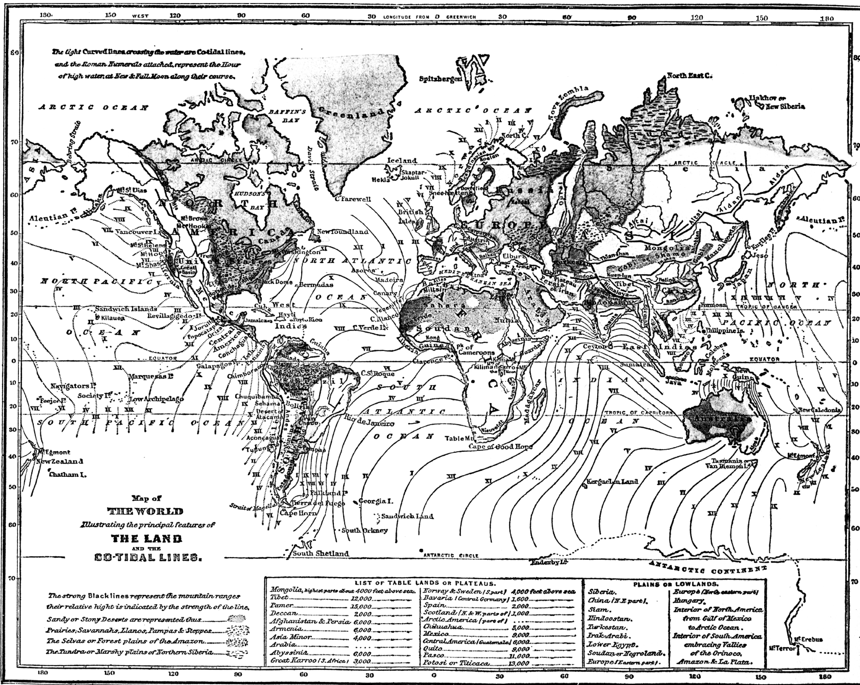
Map of the World illustrating the principal features of The Land and the Co-Tidal Lines, 1855 George W. Fitch, Outlines of Physical Geography (New York, NY: Ivison, Phinney, Blakeman & Company, 1868) Downloaded from Maps ETC , on the web at http://etc.usf.edu/maps [map #03133]
