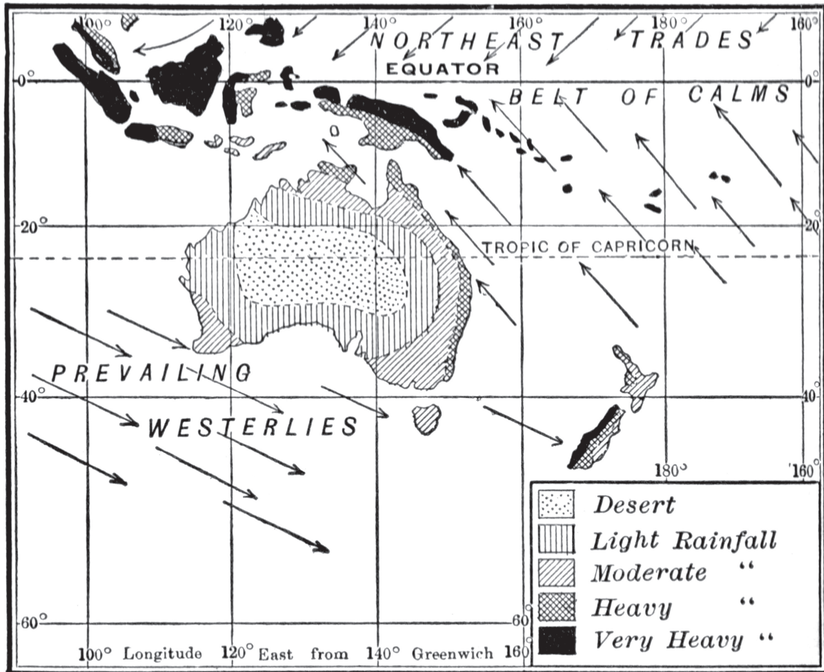
Rainfall and Wind in Oceania, 1910 Ralph S. Tarr, B.S., F.G.S.A. and Frank M. McMurry, Ph.D., New Geographies 2nd ed (New York, NY: The Macmillan Company, 1910)
