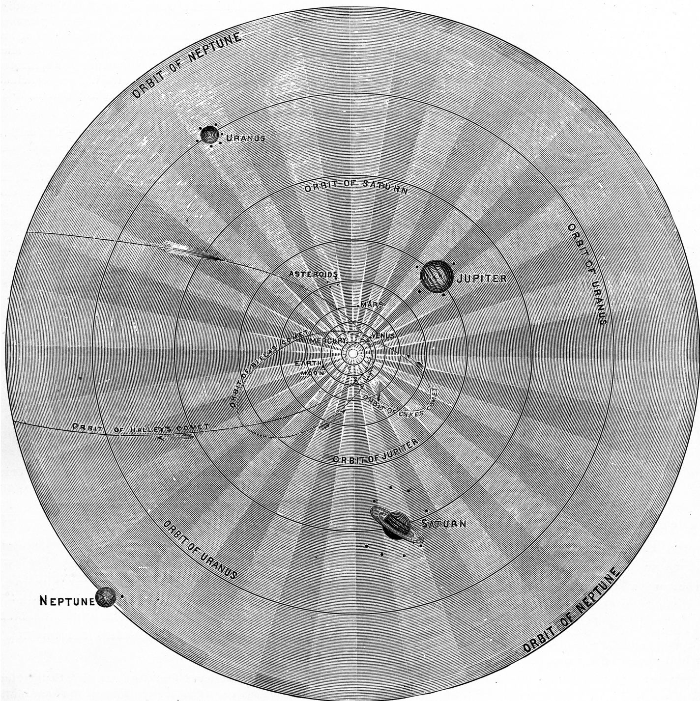
Fig. 2. The Solar System.
