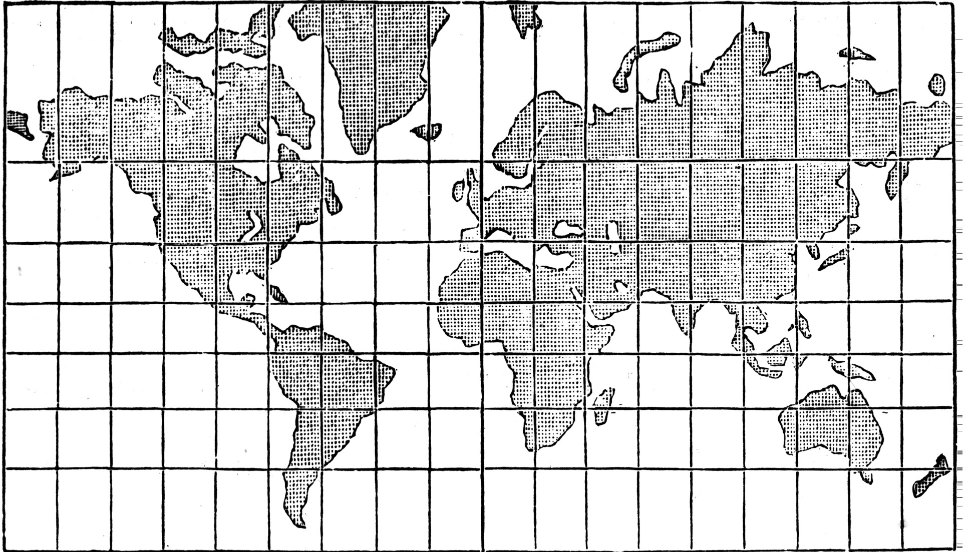
Fig. 10. The Earth on Mercator's Projection.
