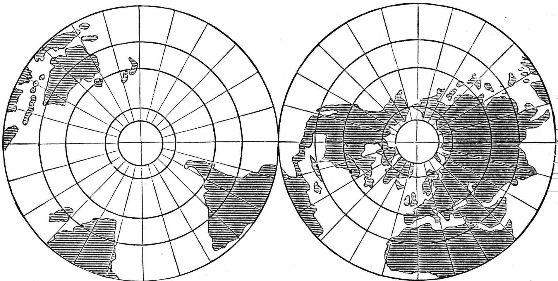
Fig. 12. The Earth on a Polar Projection.
