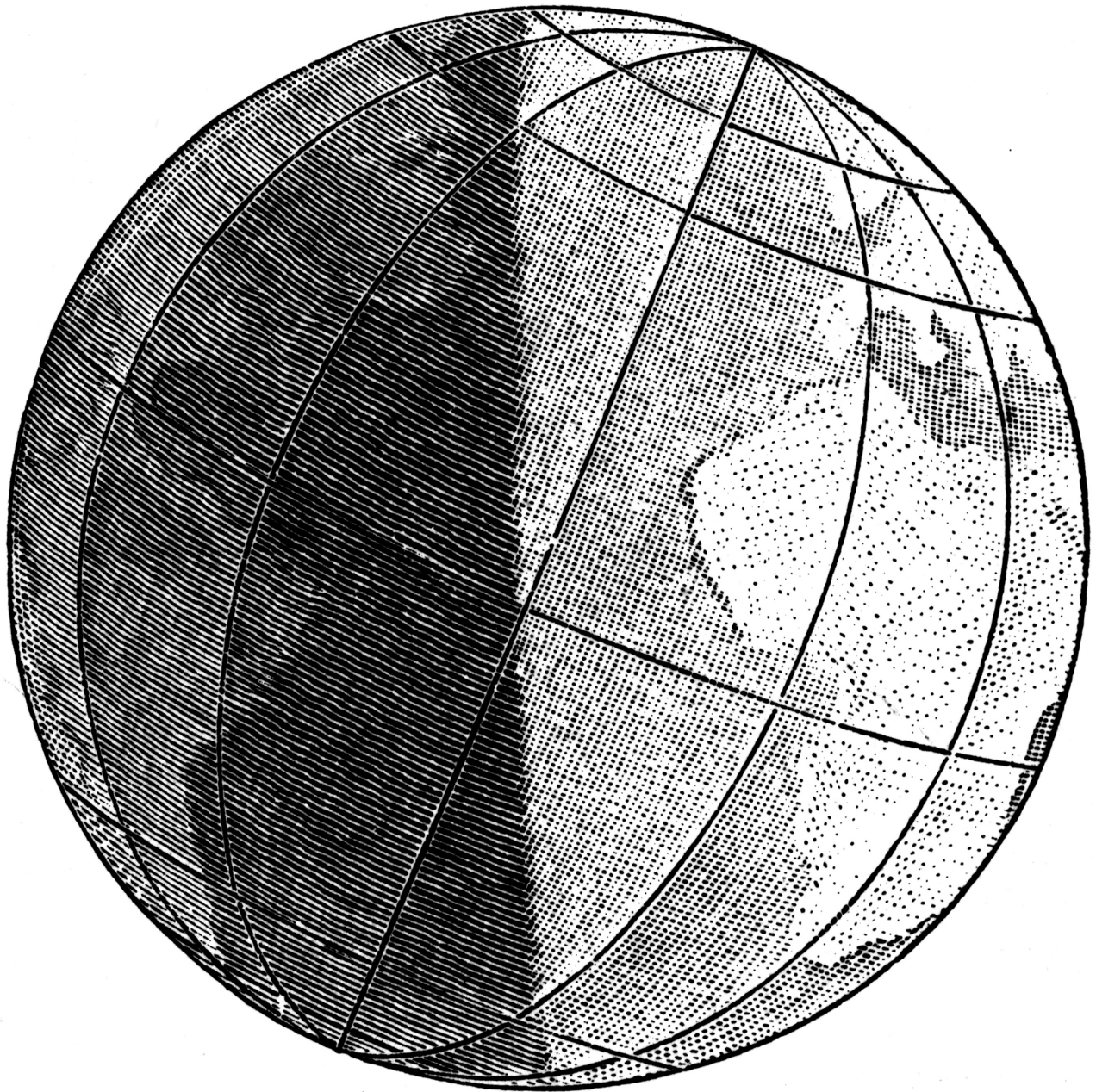
Fig. 17. The Earth at the Summer Solstice.
