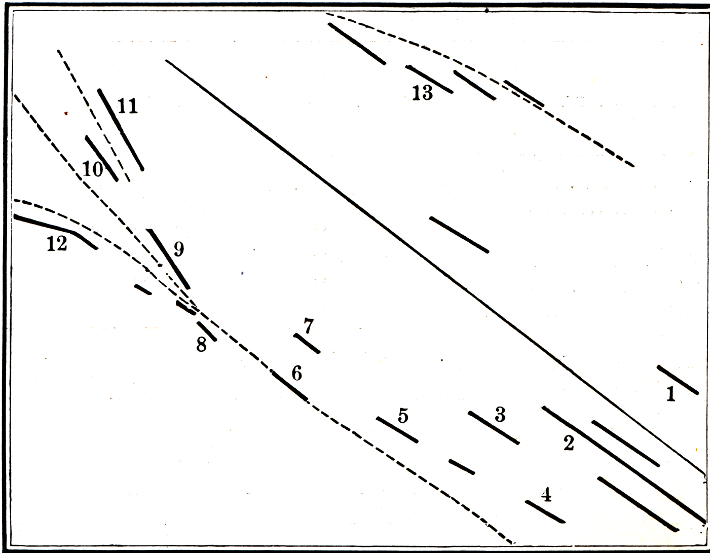
Fig. 35. Polynesian Island Chain.
