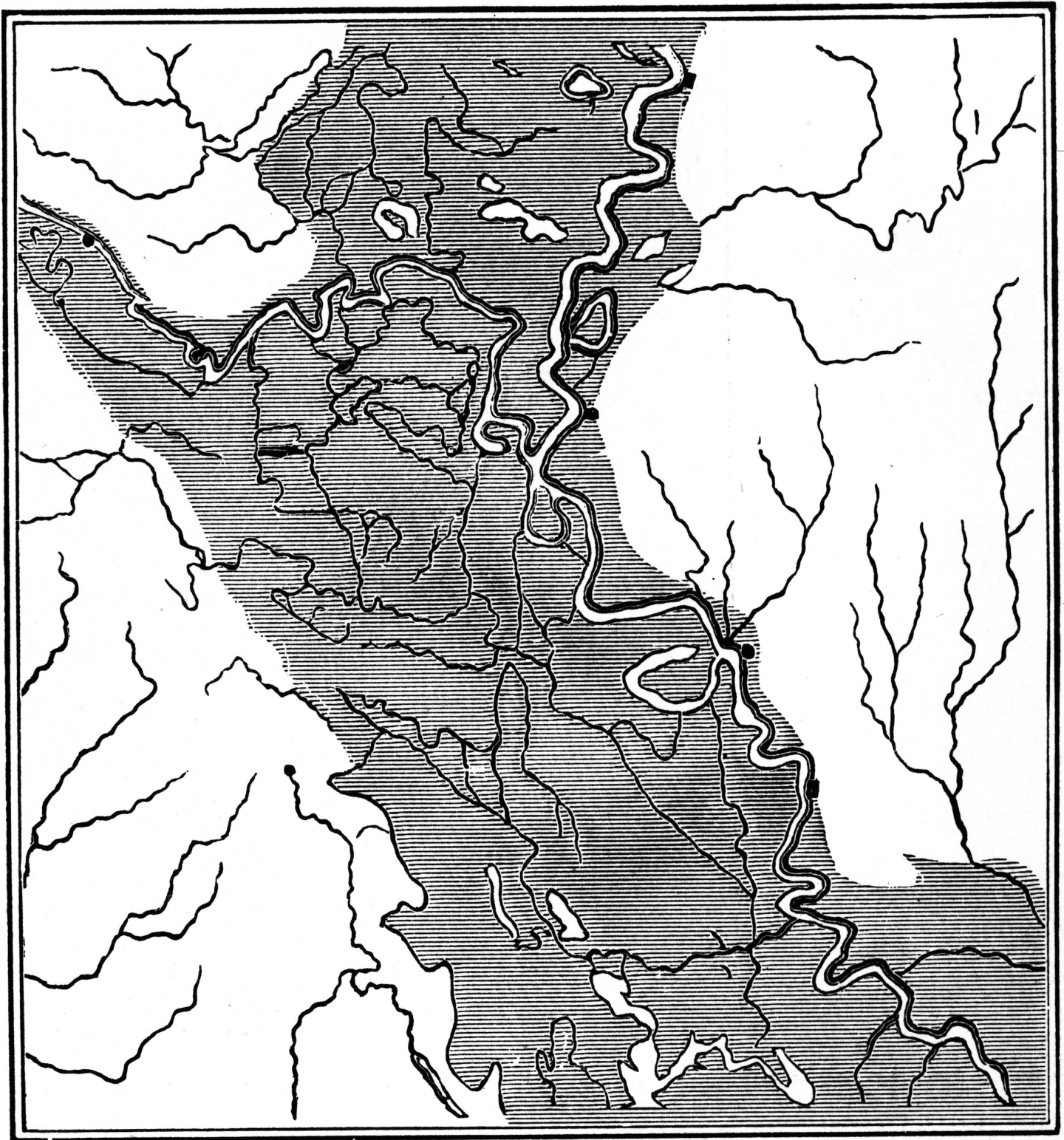
Fig. 63. Alluvial Flats of the Mississippi. (Showing deserted courses and fluviate islands and lakes.)
