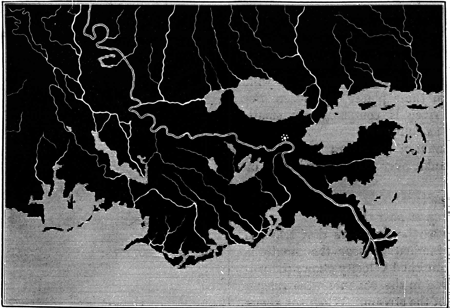
Fig. 65. Delta of the Mississippi. (After Dana.)
