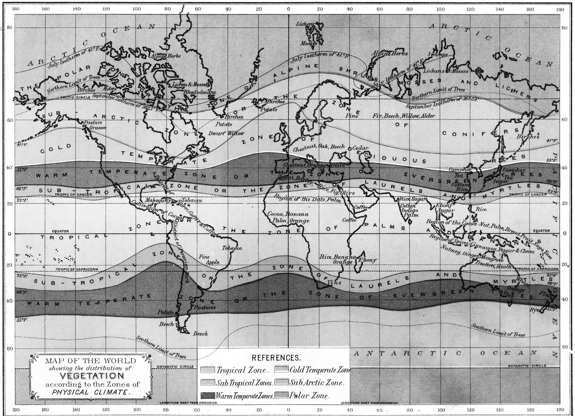
Map of the World showing the distribution of Vegetation according to the Zones of Physical Climate, 1891 Edwin J. Houston, A. M., The Elements of Physical Geography (Philadelphia, PA: Eldredge & Brother, 1891) Downloaded from Maps ETC , on the web at http://etc.usf.edu/maps [map #02613]
