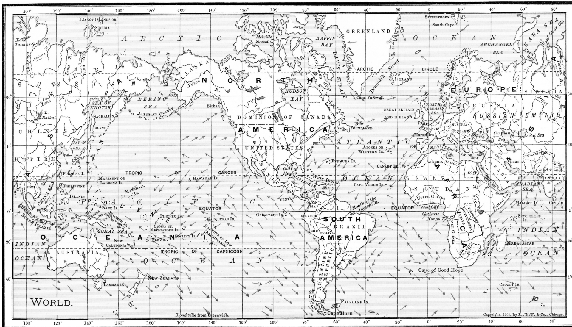
1. MAP OF WORLD SHOWING WINDS FOR JANUARY. (Fig. 65.)
