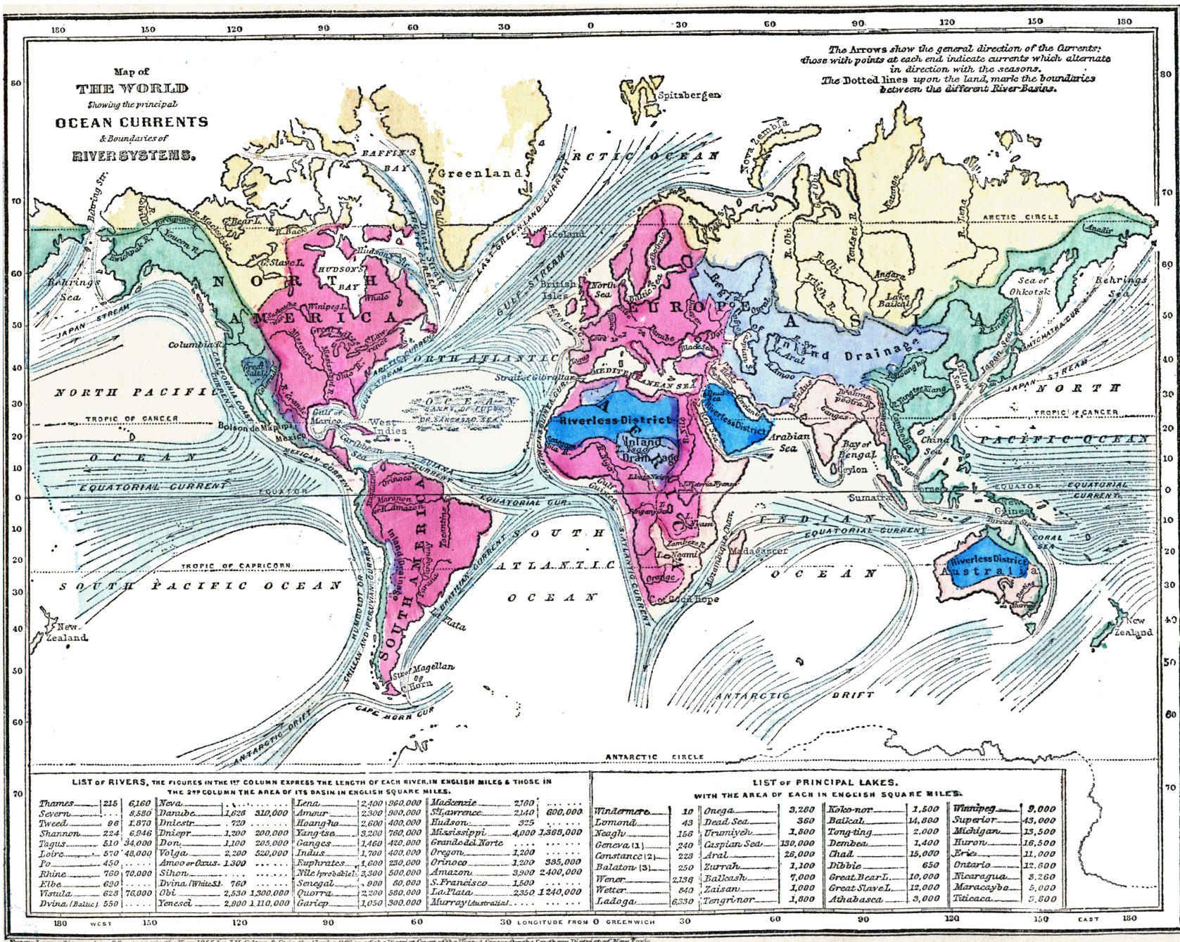
Map of the World showing the principal Ocean Currents & boundaries of River Systems, 1855 George W. Fitch, Outlines of Physical Geography (New York, NY: Ivison, Phinney, Blakeman & Company, 1868) Downloaded from Maps ETC, on the web at http://etc.usf.edu/maps [map #03135]
