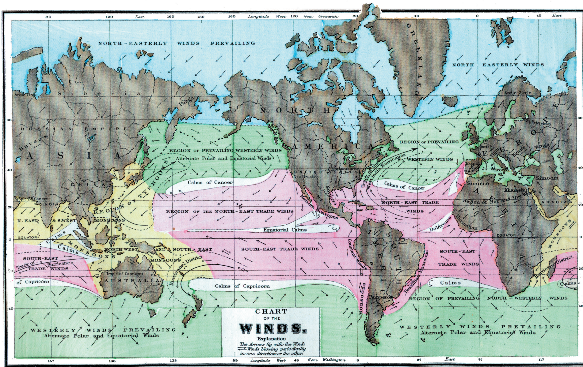
Chart of Winds, 1873
