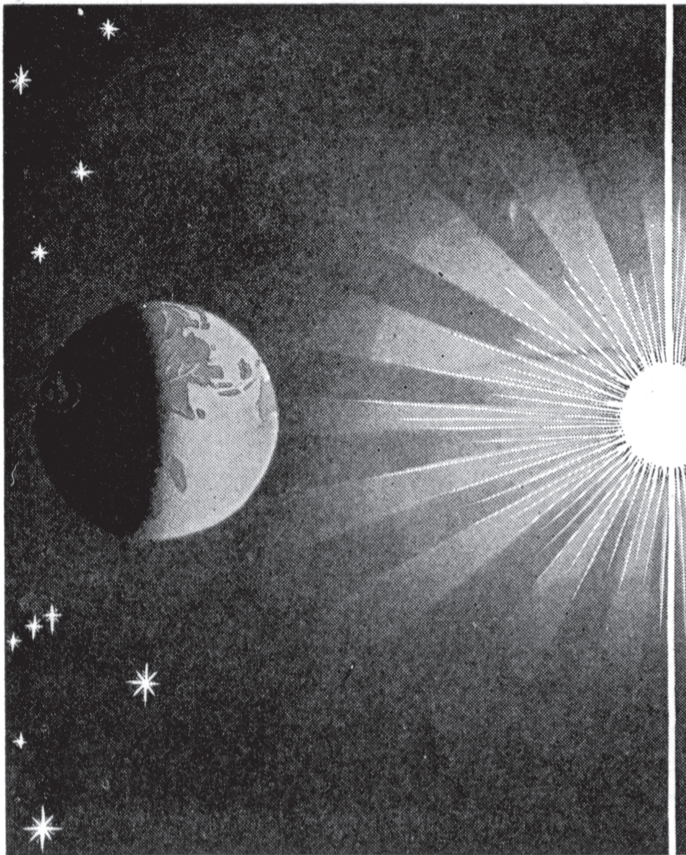
THE EARTH ON A WINTER'S NIGHT IN ENGLAND
