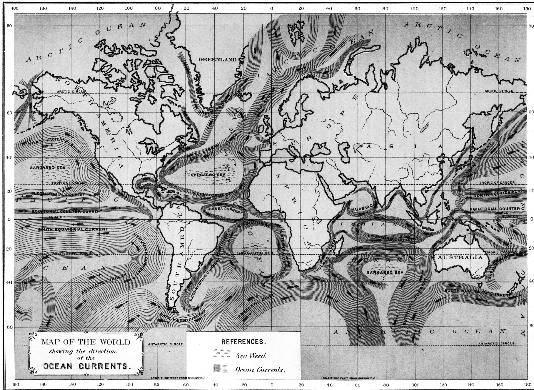
Map of the World showing the direction of the Ocean Currents, 1891 Edwin J. Houston, A. M., The Elements of Physical Geography (Philadelphia, PA: Eldredge & Brother, 1891) Downloaded from Maps ETC , on the web at http://etc.usf.edu/maps [map #02609]
