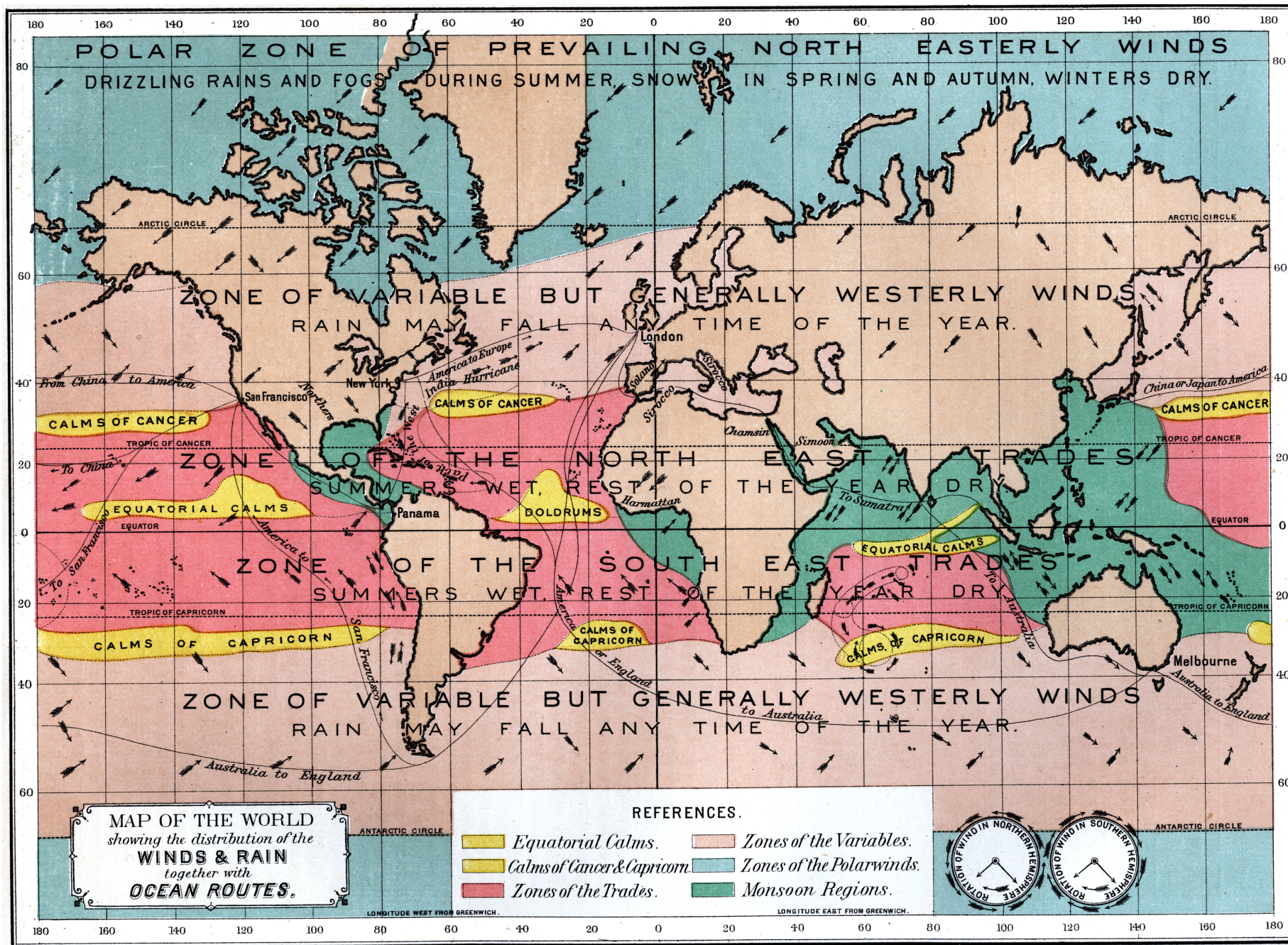
Map of the World showing the distribution of the Wind & Rain together with Ocean Routes, 1891 Edwin J. Houston, A. M., The Elements of Physical Geography (Philadelphia, PA: Eldredge & Brother, 1891) Downloaded from Maps ETC , on the web at http://etc.usf.edu/maps [map #02611]
