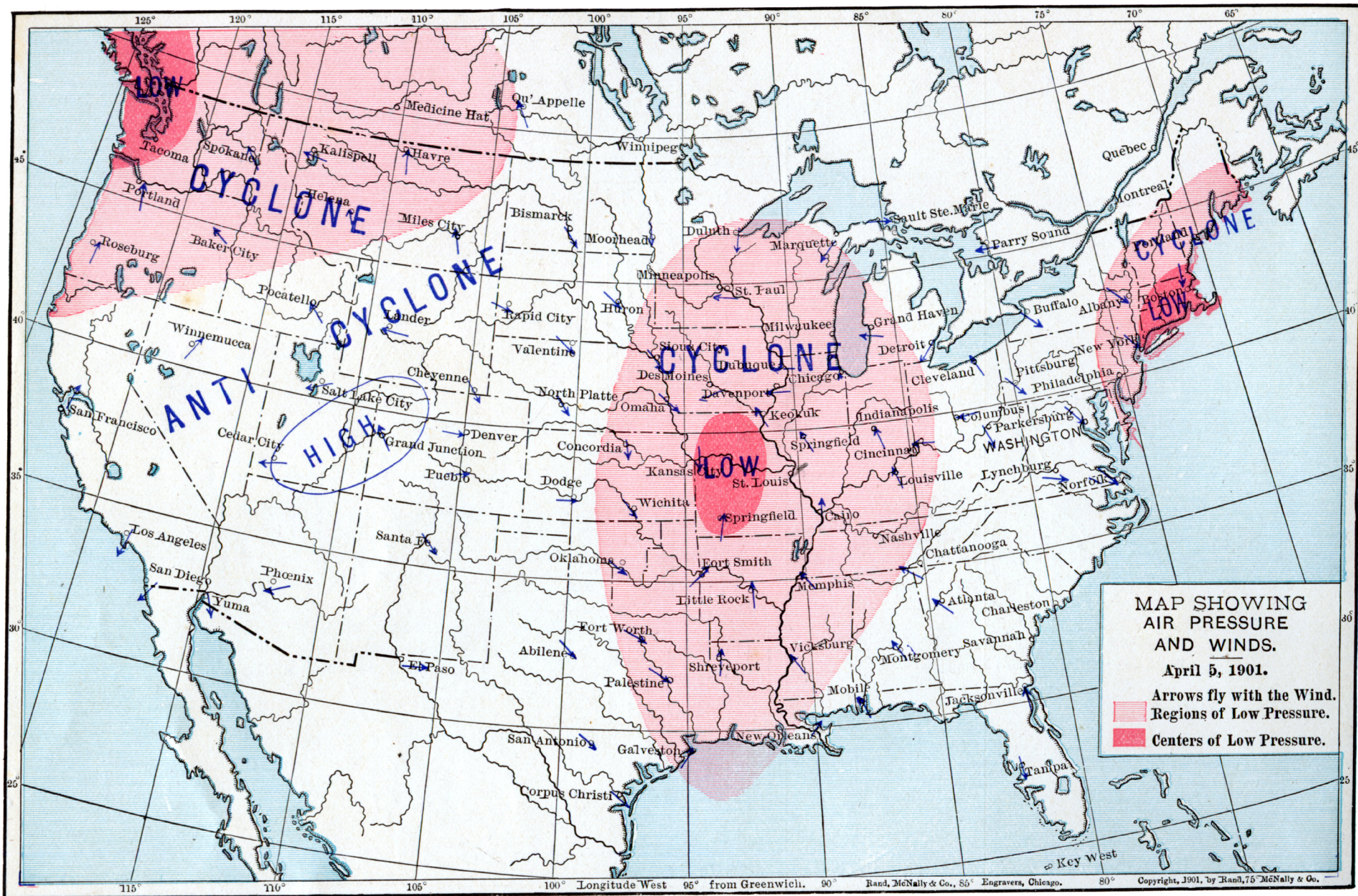
MAP SHOWING AIR PRESSURE AND WINDS, APRIL 5, 1901. (Fig. 71.)
