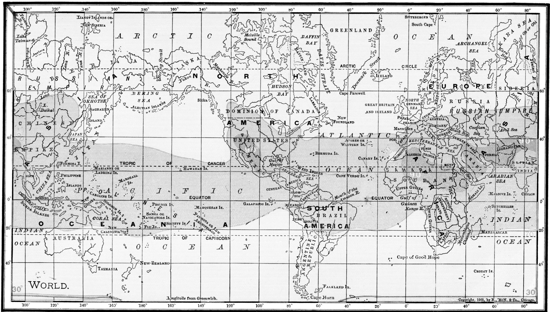
MAP SHOWING ISOOTHERMS FOR JULY. (Fig. 78.)
