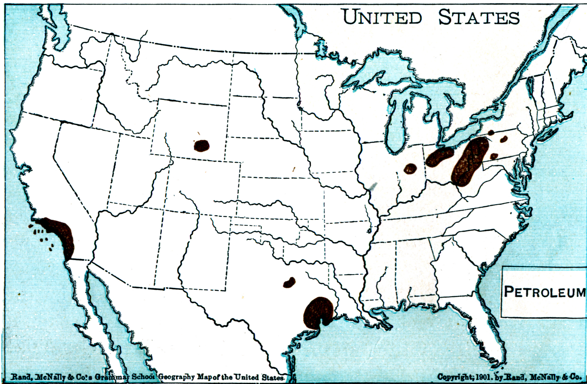
MAP SHOWING PRODUCTION OF PETROLEUM. (Fig. 152.)
