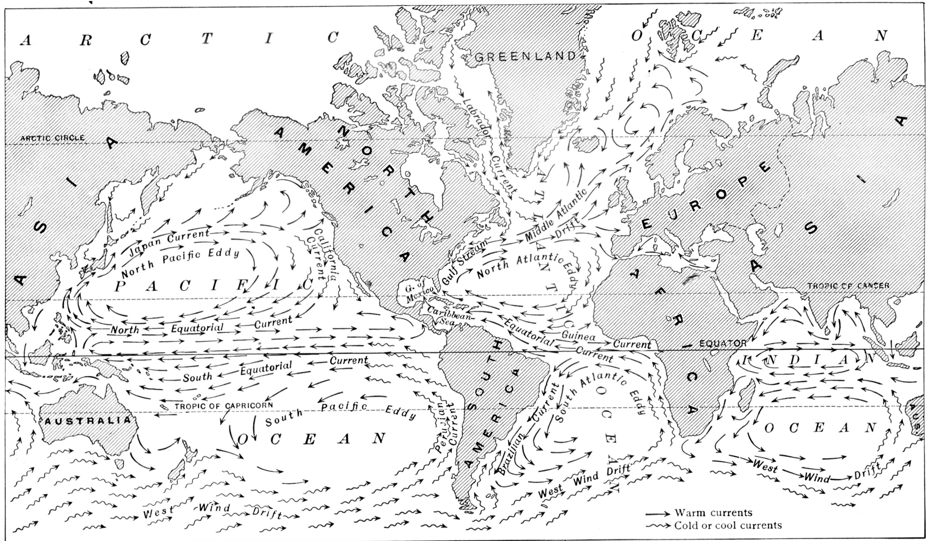
FIG. 255. Ocean currents.
