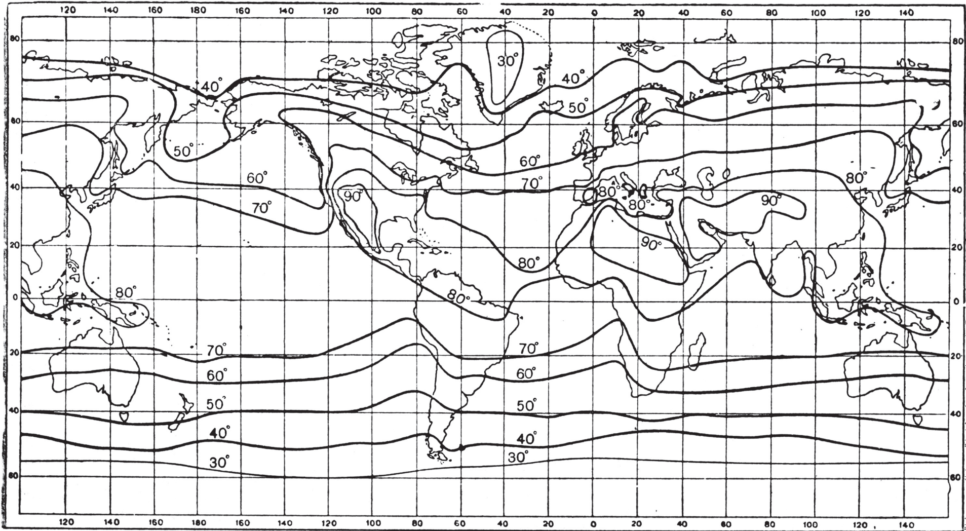
Fig. 4.—JULY ISOTHERMS
