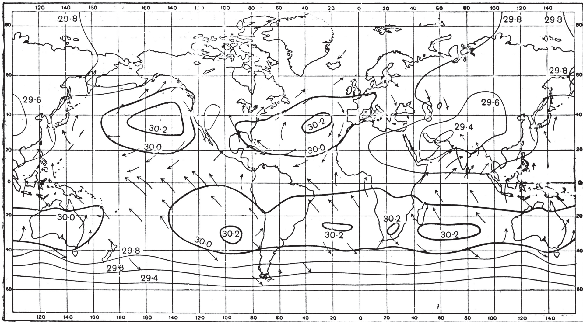
Fig. 6.—JULY ISOBARS
