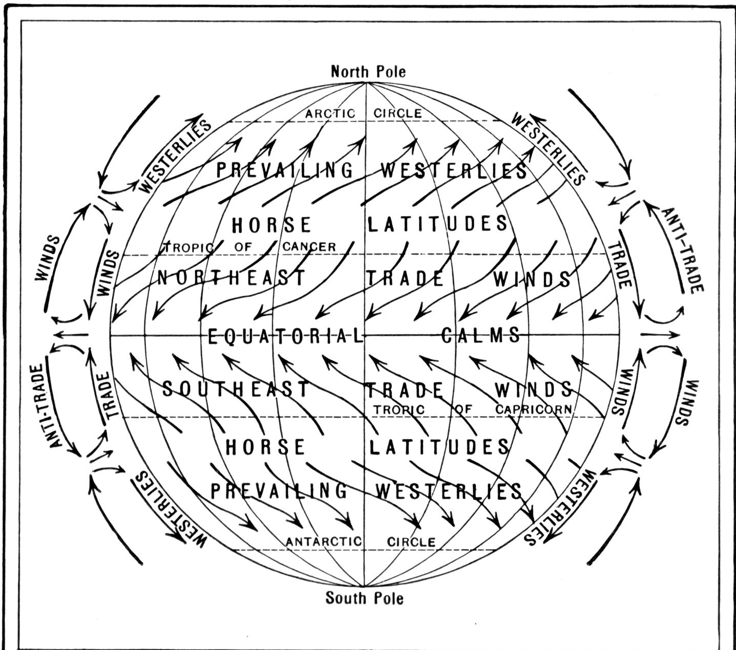
Fig. 370. Winds on the earth's surface; also vertical section of the atmosphere, on a larger scale, showing circulation
