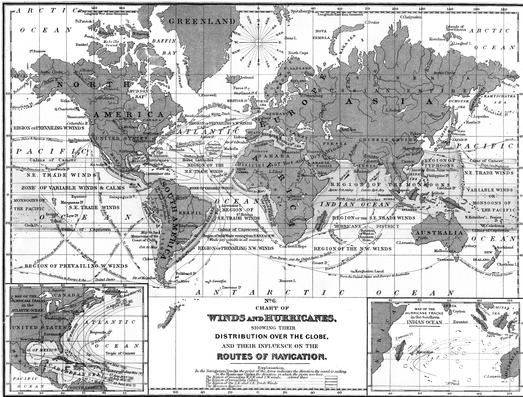
Chart of Winds and Hurricanes, 1890
