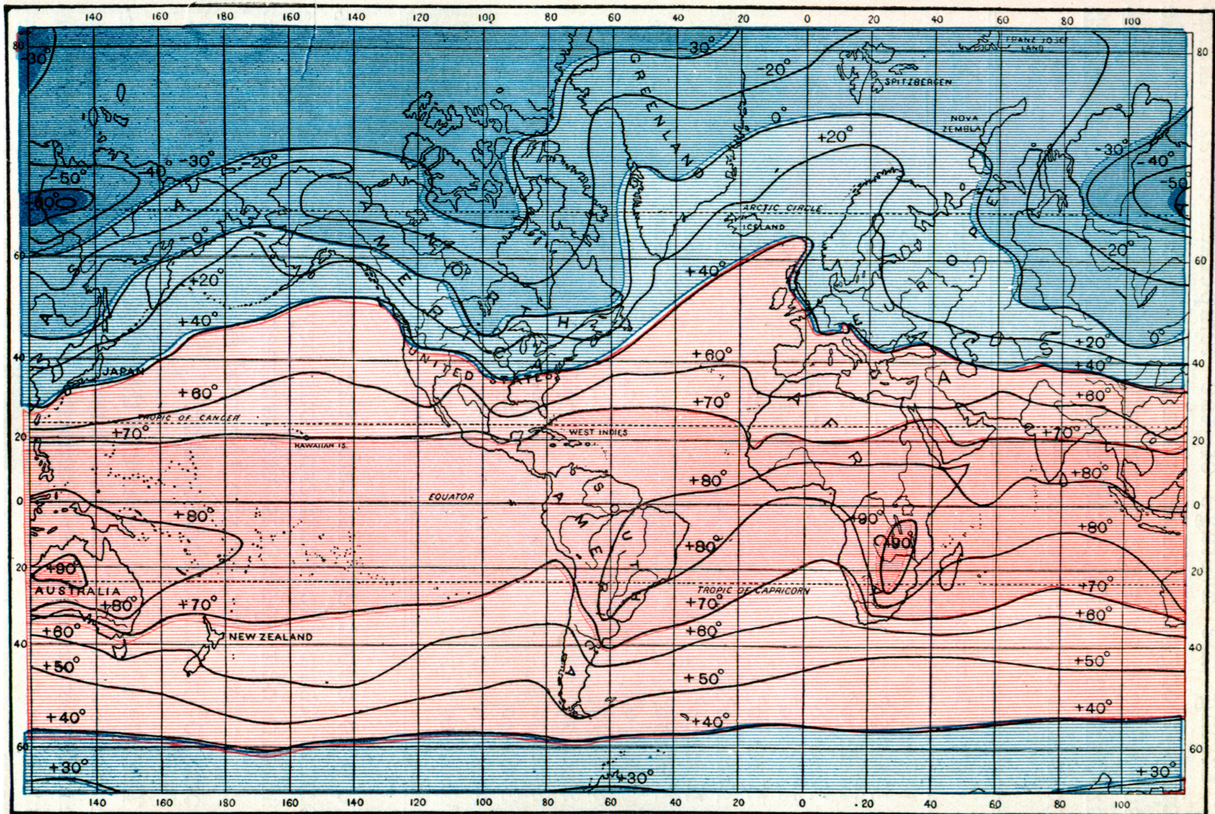
FIG. 10. — AVERAGE TEMPERATURE FOR JANUARY (AFTER BUCHAN).
