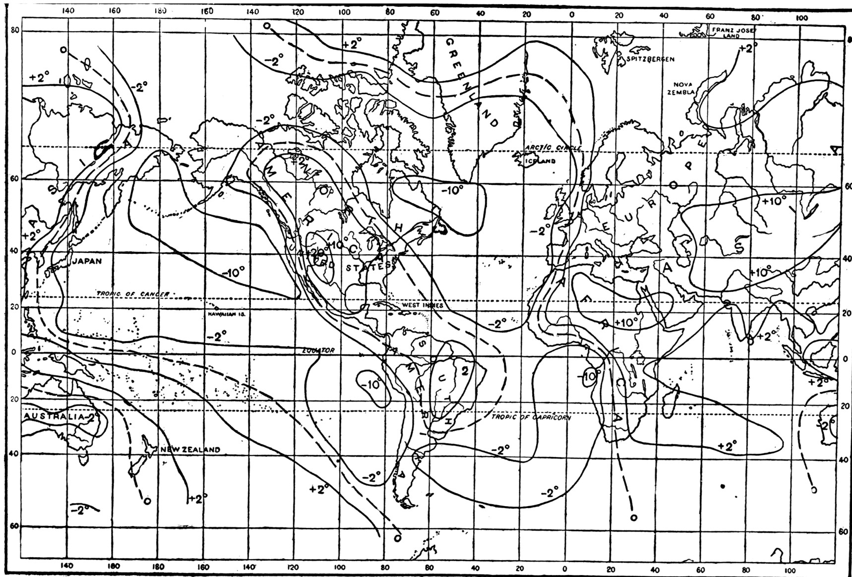
FIG. 13. — IS-ABNORMAL TEMPERATURES FOR JULY (AFTER BATCHELDER).
