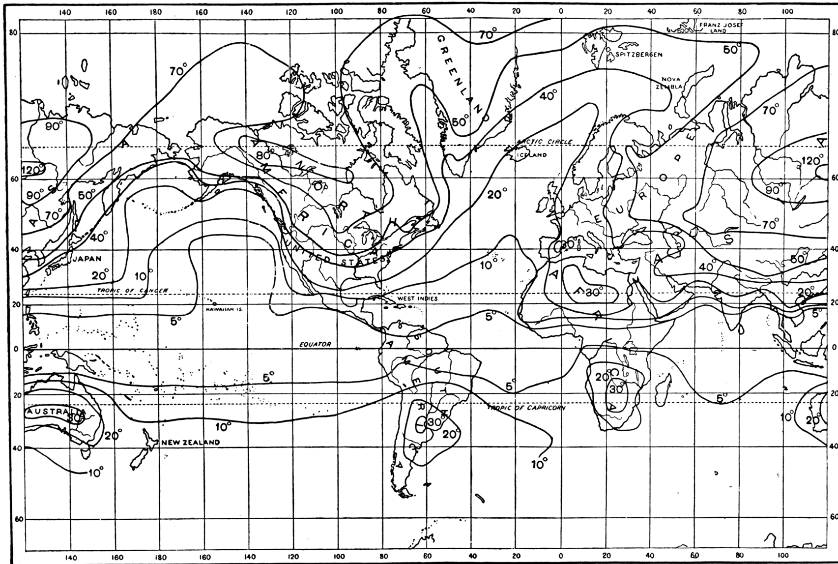
FIG. 14. — ANNUAL RANGE OF AVERAGE MONTHLY TEMPERATURE (AFTER CONOLLY).
