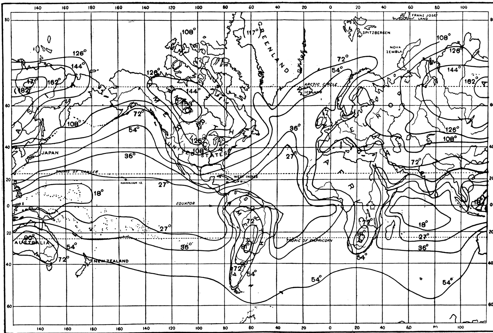
FIG. 17. — AVERAGE EXTREME TEMPERATURE OSCILLATION DURING THE YEAR (AFTER VAN BEBBER).
