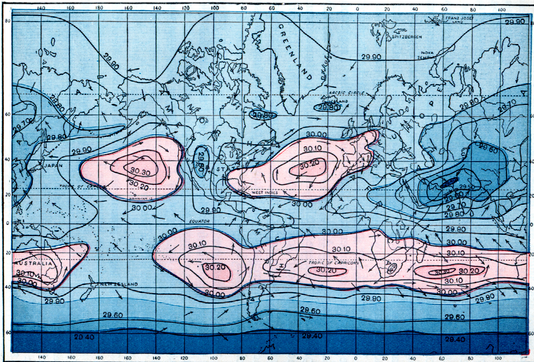
FIG. 27. — ISOBARS (AT SEA LEVEL) FOR JULY (AFTER BUCHAN).
